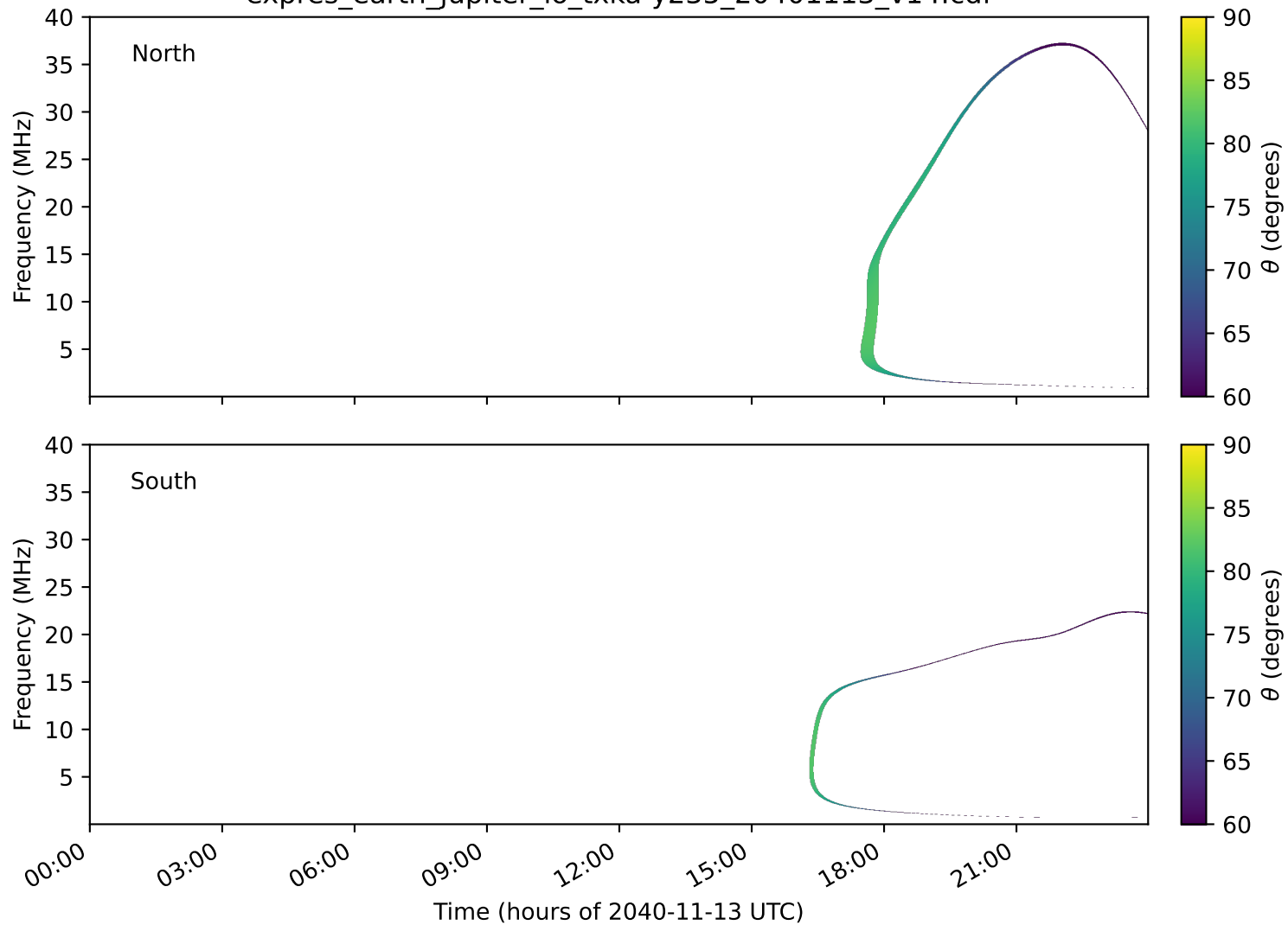
expres_earth_jupiter_io_txka-y235_20401113_v14.cdf
