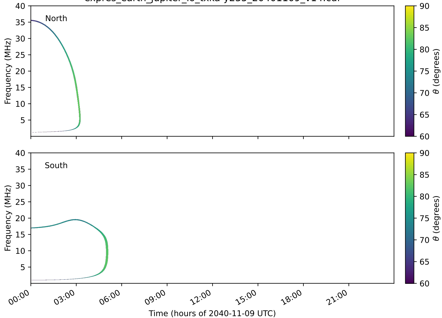
expres_earth_jupiter_io_txka-y235_20401109_v14.cdf
