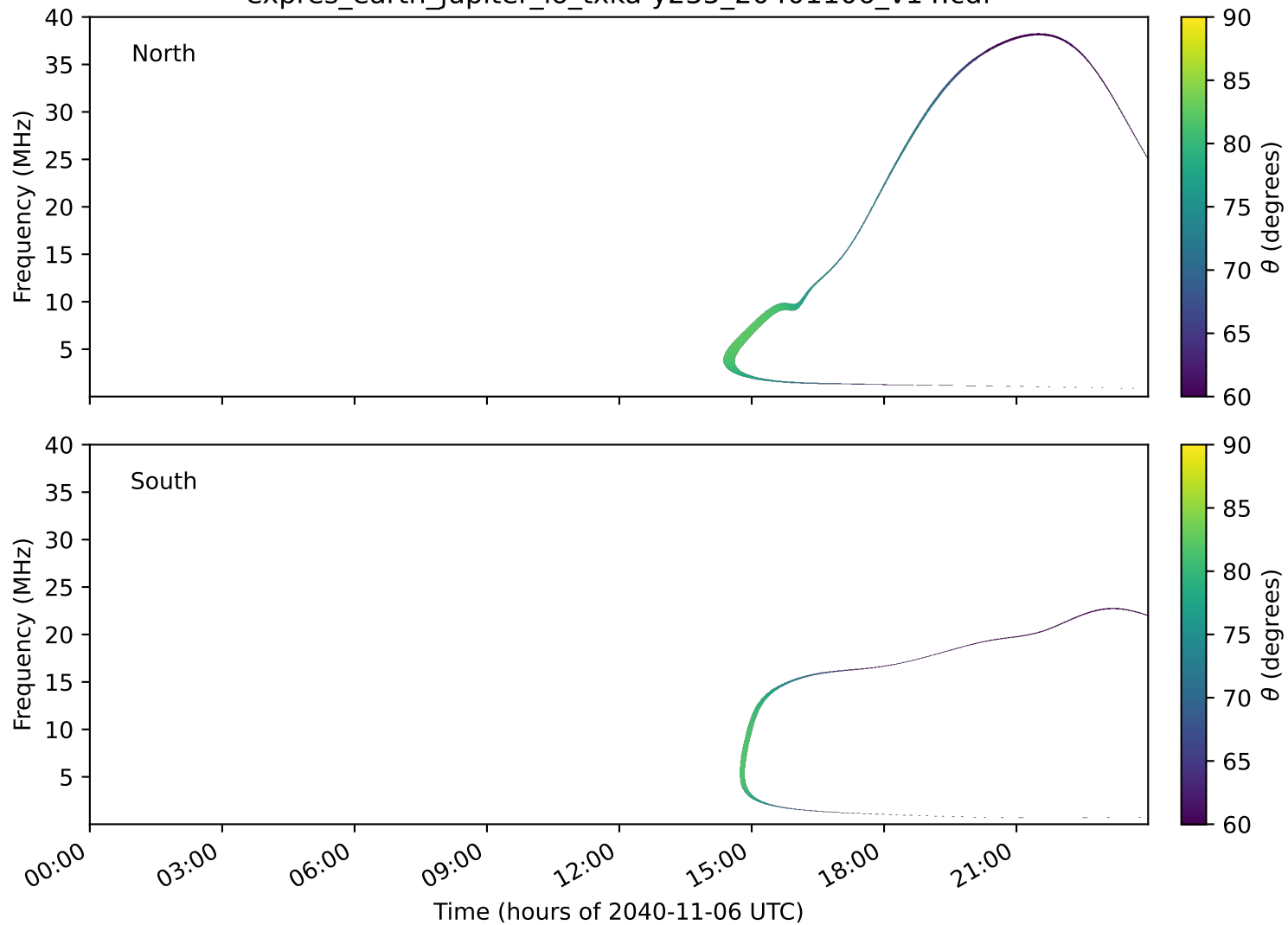
expres_earth_jupiter_io_txka-y235_20401106_v14.cdf
