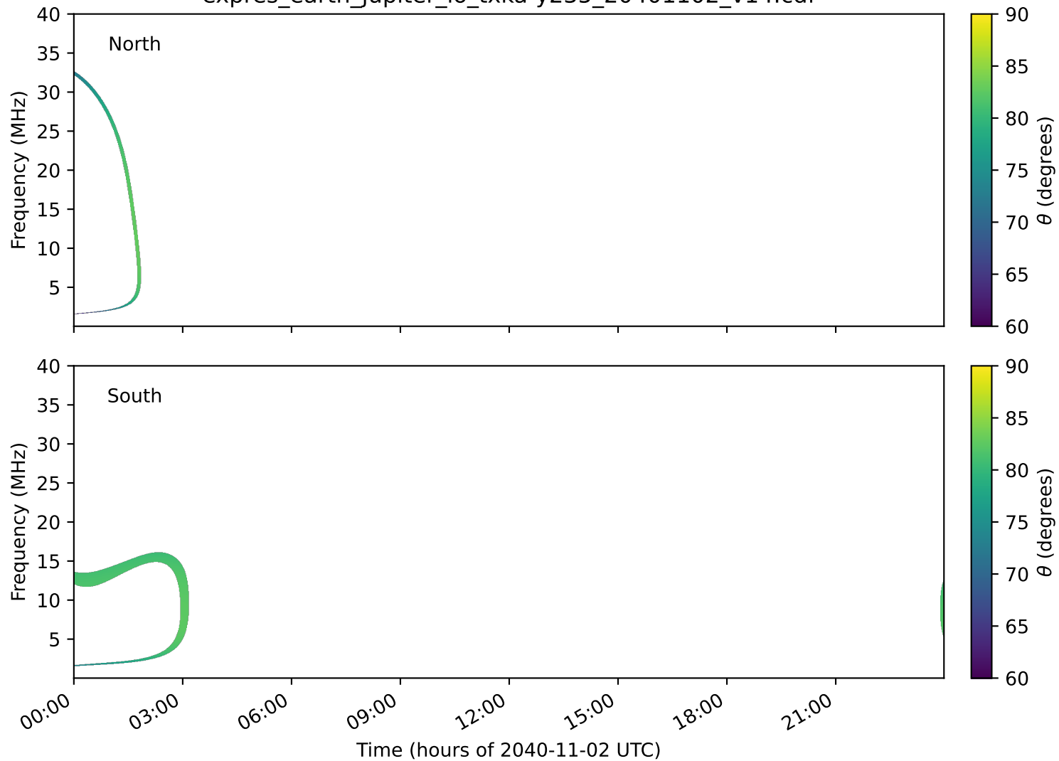
expres_earth_jupiter_io_txka-y235_20401102_v14.cdf
