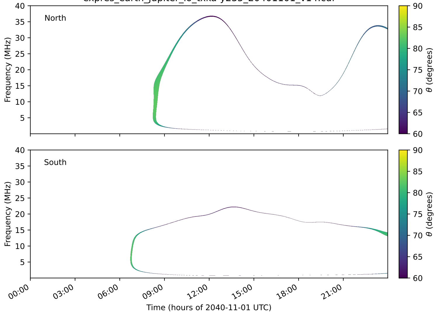
expres_earth_jupiter_io_txka-y235_20401101_v14.cdf
