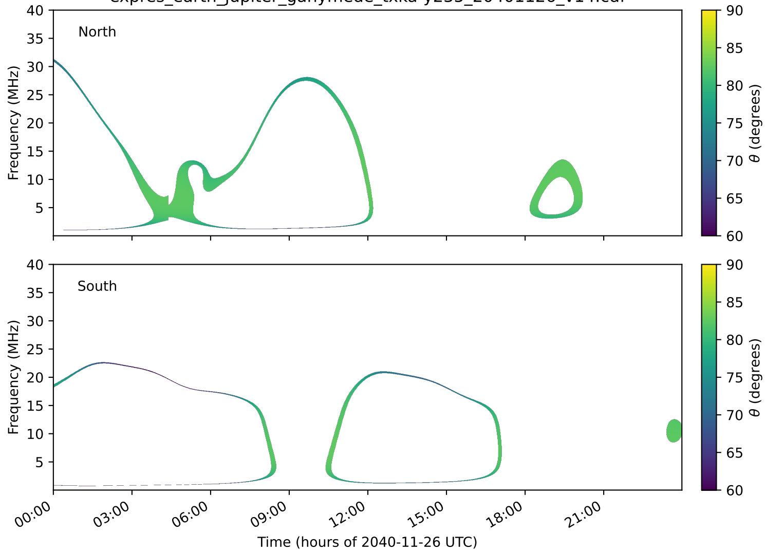
expres_earth_jupiter_ganymede_txka-y235_20401126_v14.cdf
