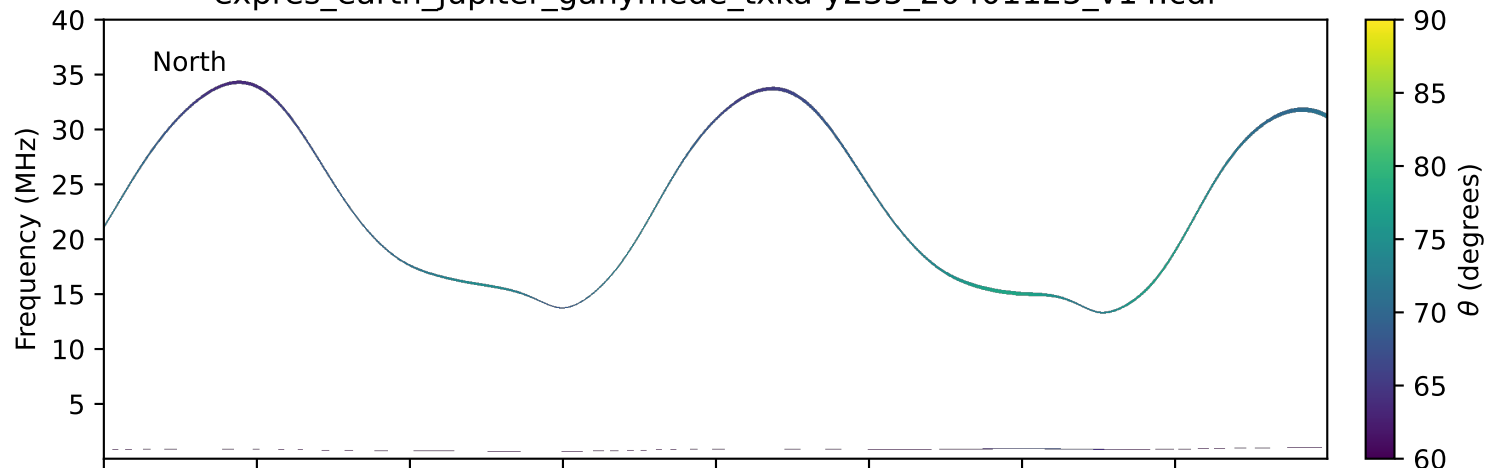
expres_earth_jupiter_ganymede_txka-y235_20401125_v14.cdf
