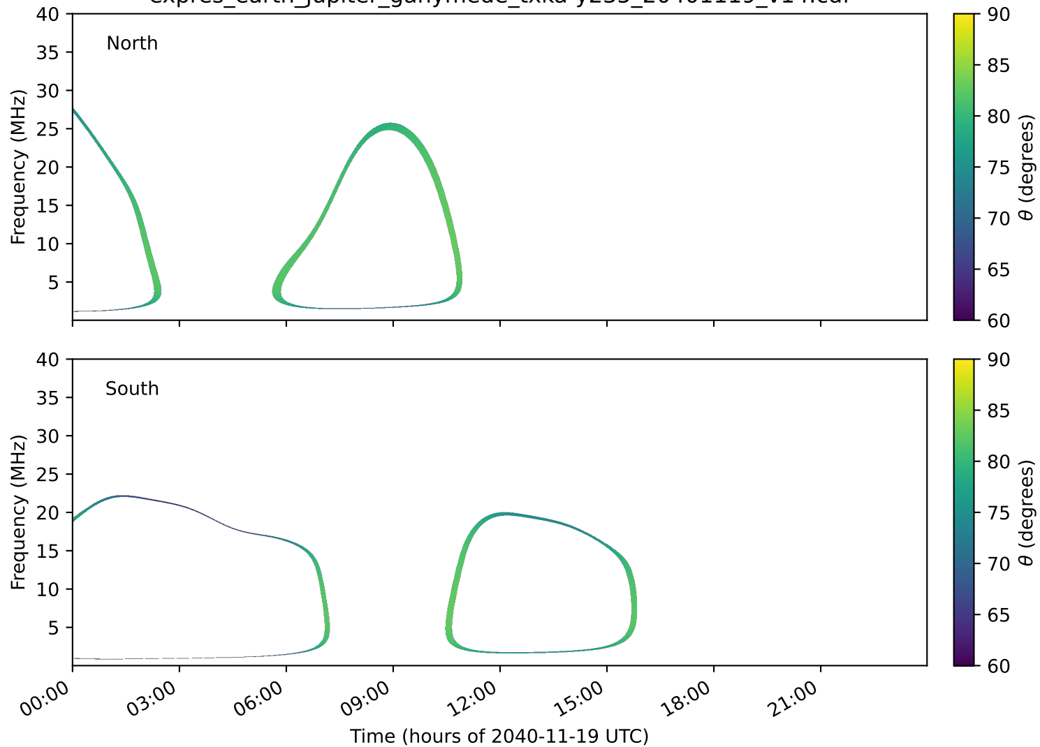
expres_earth_jupiter_ganymede_txka-y235_20401119_v14.cdf
