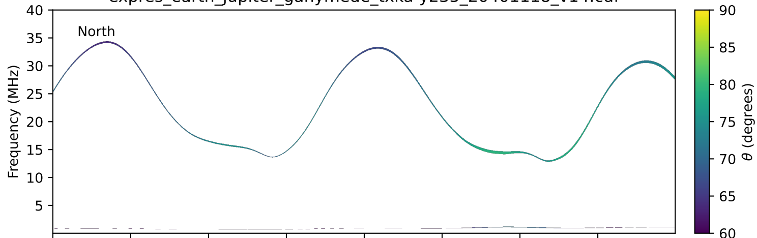
expres_earth_jupiter_ganymede_txka-y235_20401118_v14.cdf
