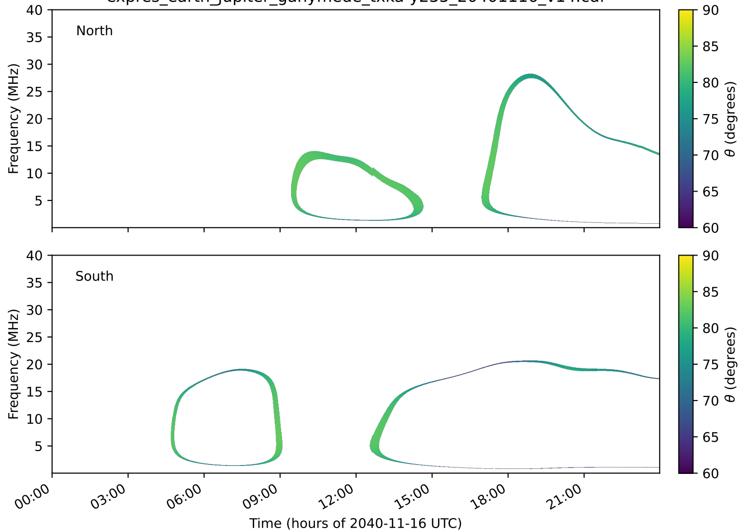
expres_earth_jupiter_ganymede_txka-y235_20401116_v14.cdf
