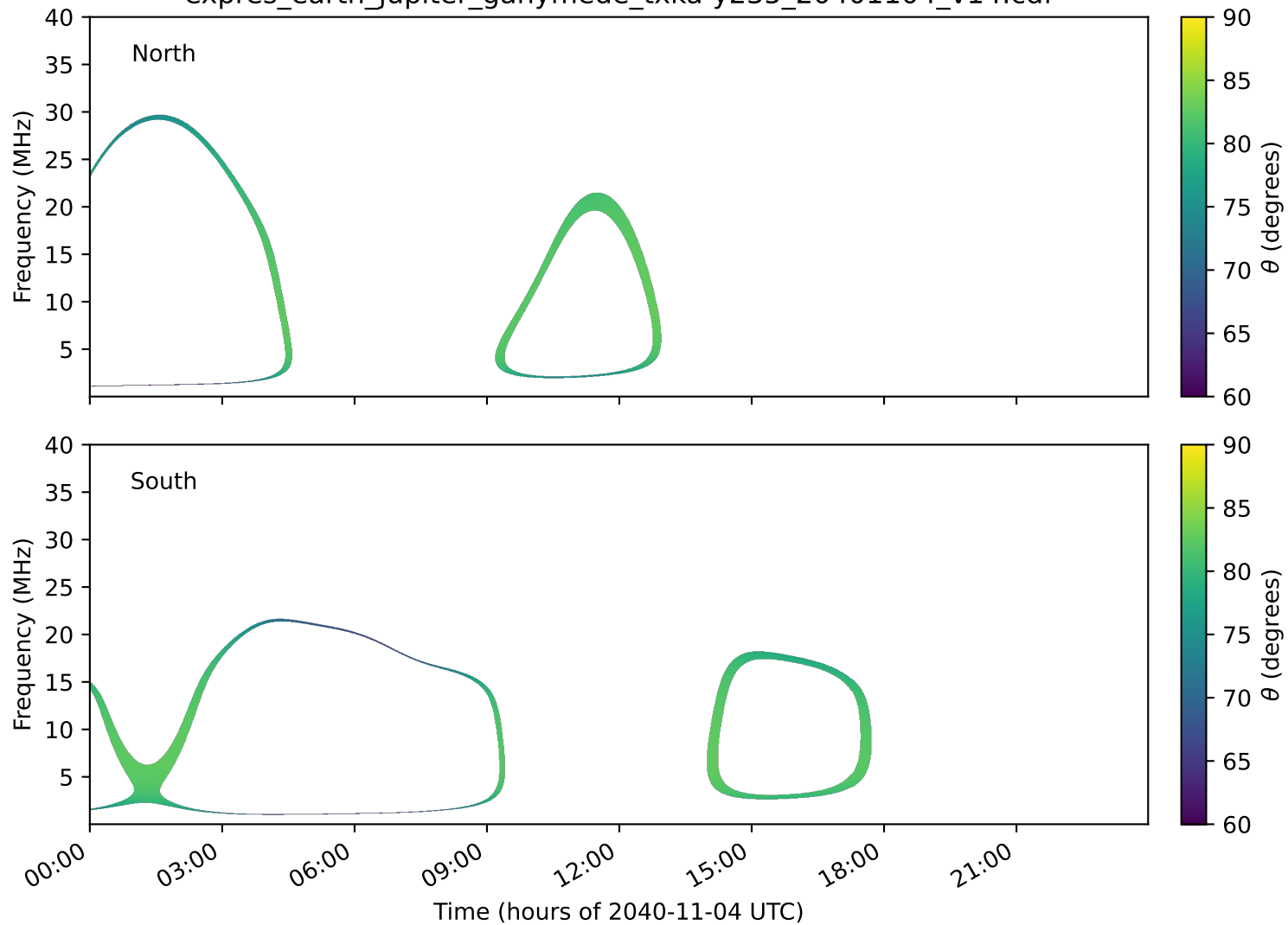
expres_earth_jupiter_ganymede_txka-y235_20401104_v14.cdf
