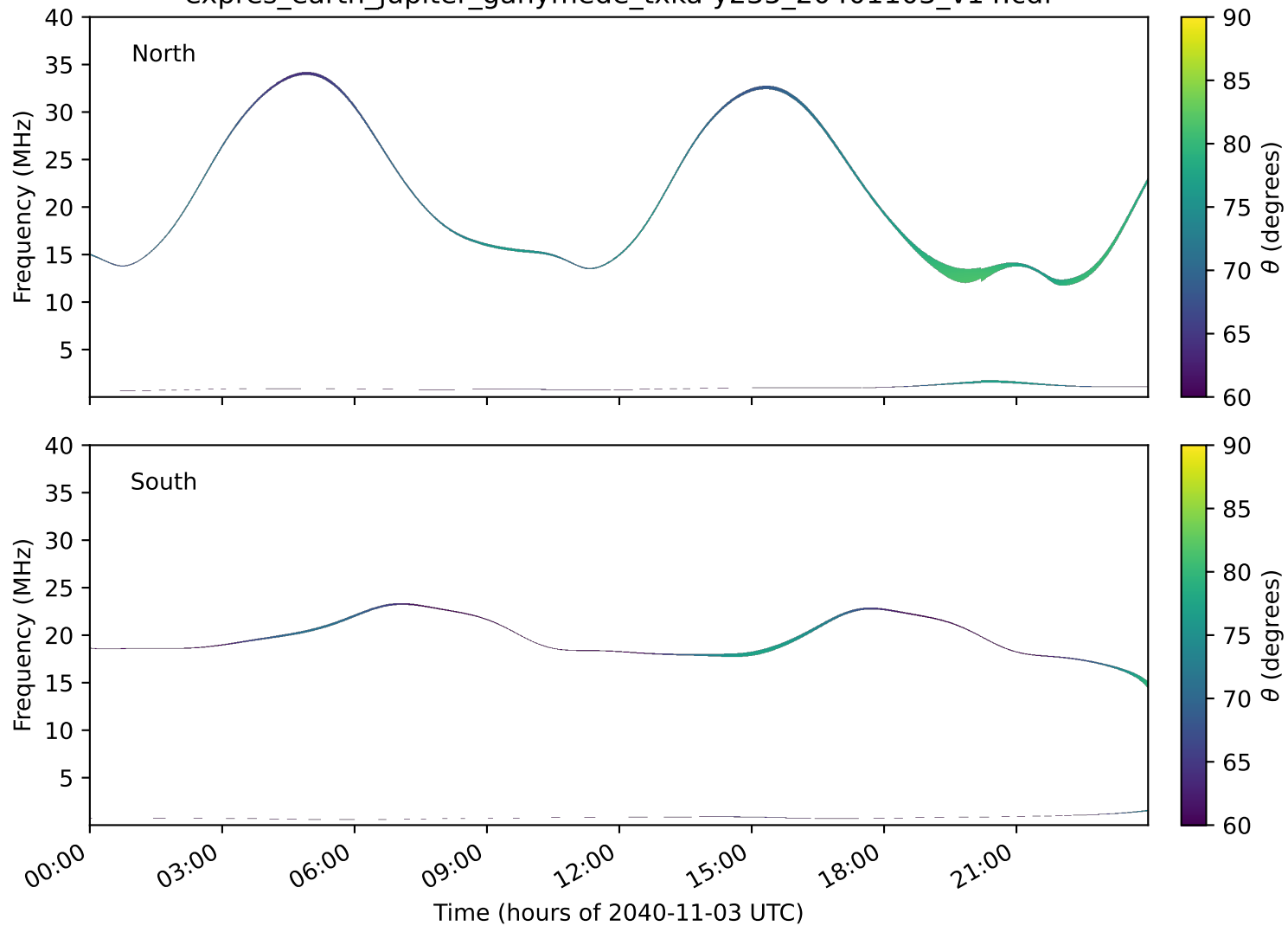
expres_earth_jupiter_ganymede_txka-y235_20401103_v14.cdf
