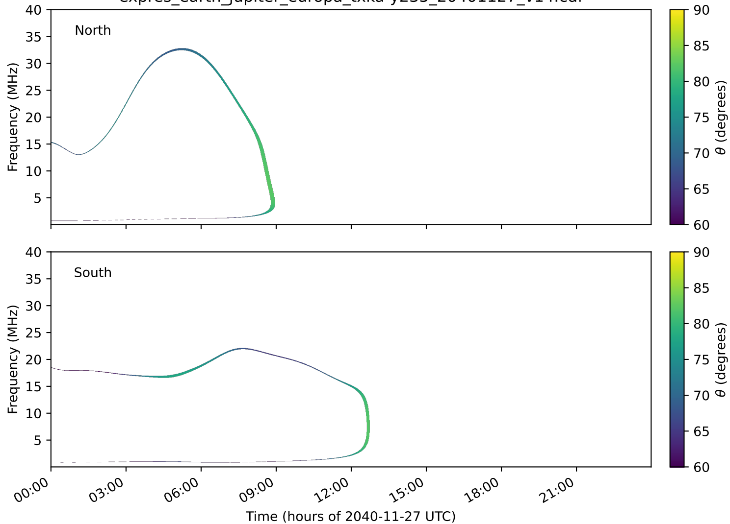
expres_earth_jupiter_europa_txka-y235_20401127_v14.cdf
