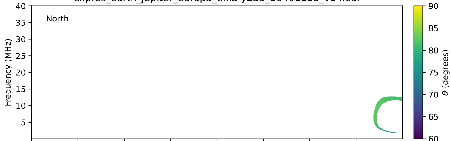
expres_earth_jupiter_europa_txka-y235_20401125_v14.cdf
