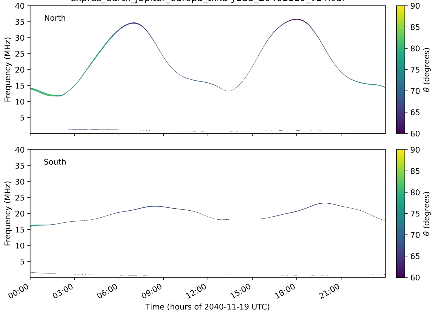
expres_earth_jupiter_europa_txka-y235_20401119_v14.cdf
