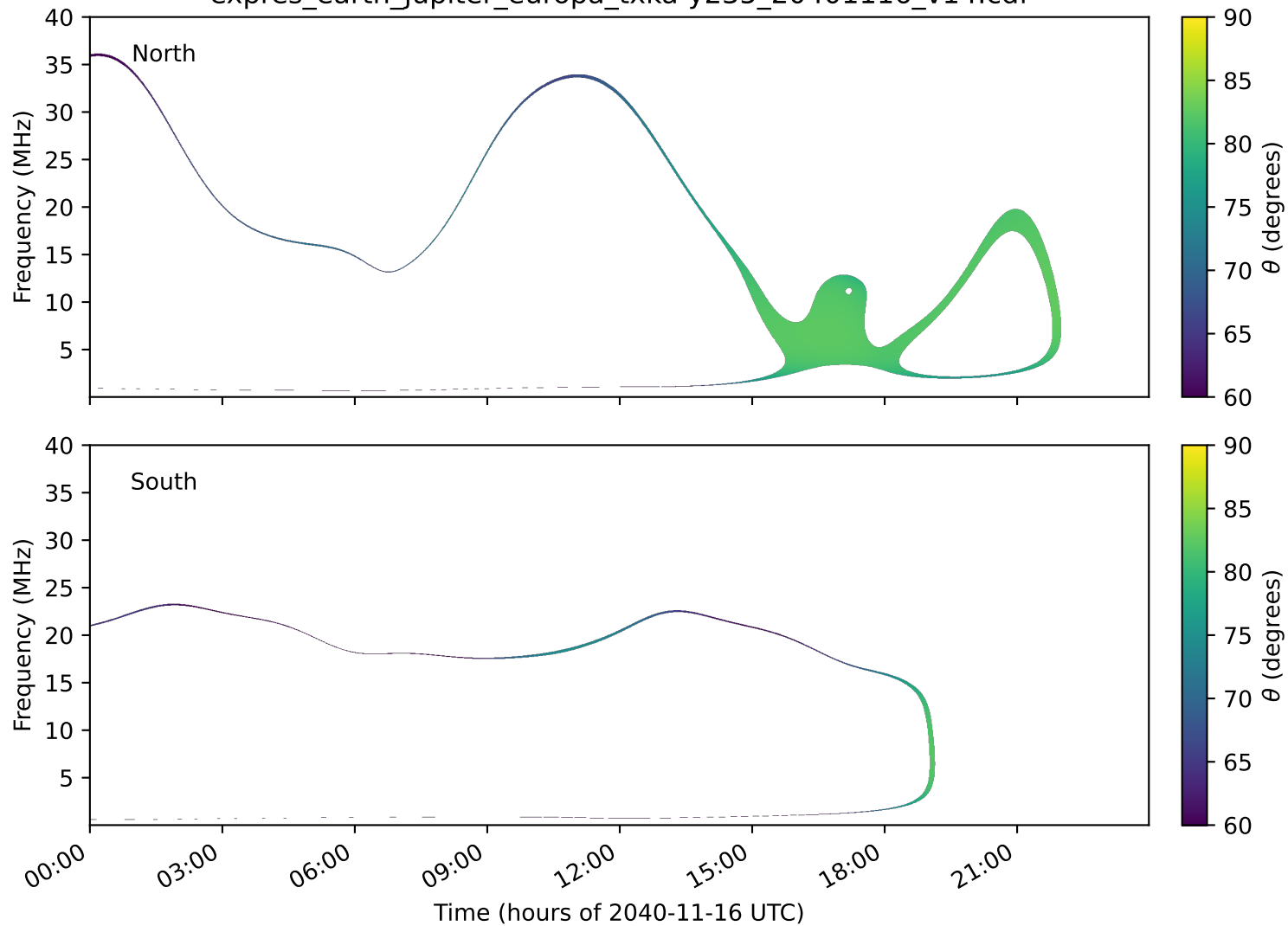
expres_earth_jupiter_europa_txka-y235_20401116_v14.cdf
