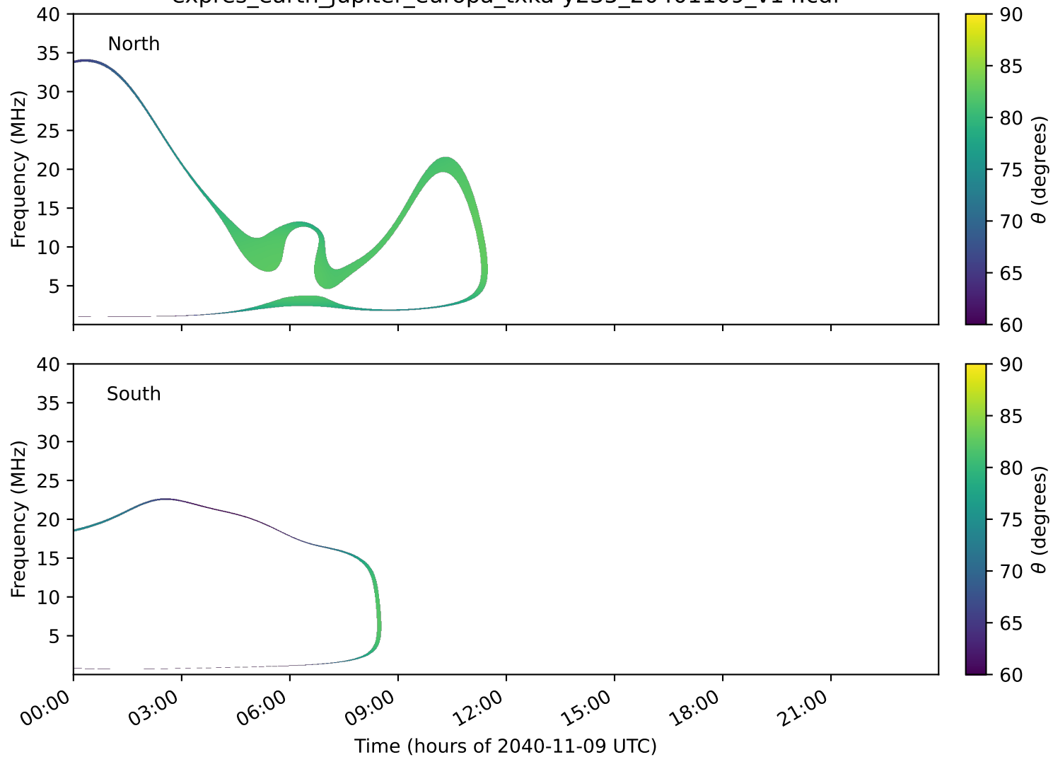
expres_earth_jupiter_europa_txka-y235_20401109_v14.cdf
