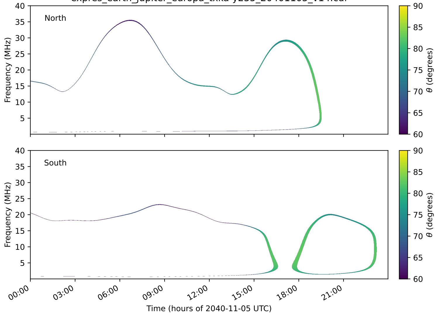
expres_earth_jupiter_europa_txka-y235_20401105_v14.cdf
