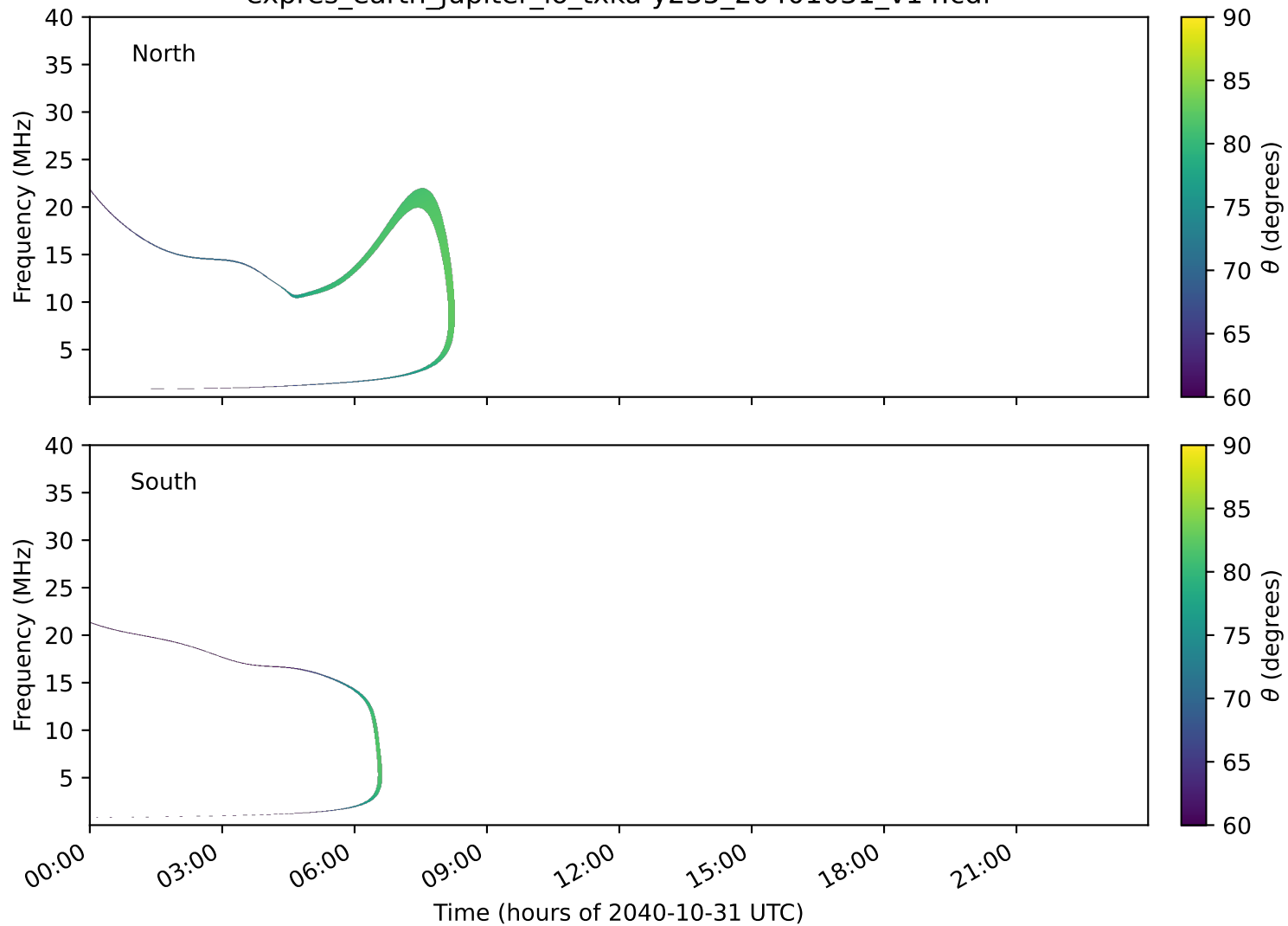
expres_earth_jupiter_io_txka-y235_20401031_v14.cdf
