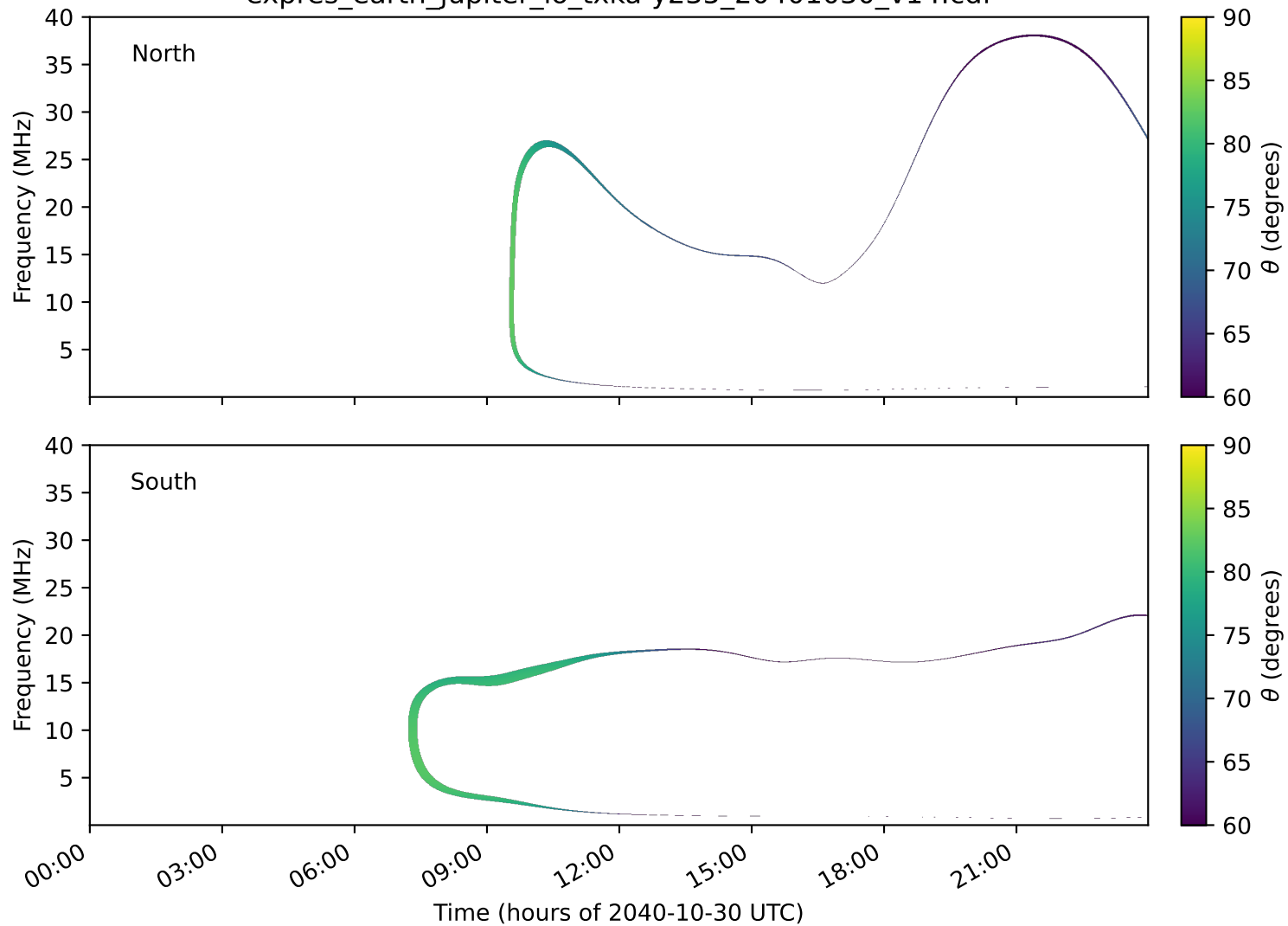
expres_earth_jupiter_io_txka-y235_20401030_v14.cdf
