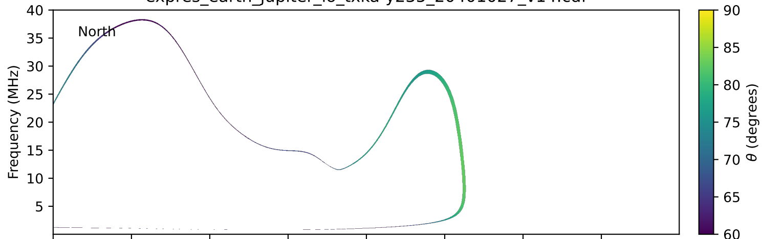
expres_earth_jupiter_io_txka-y235_20401027_v14.cdf
