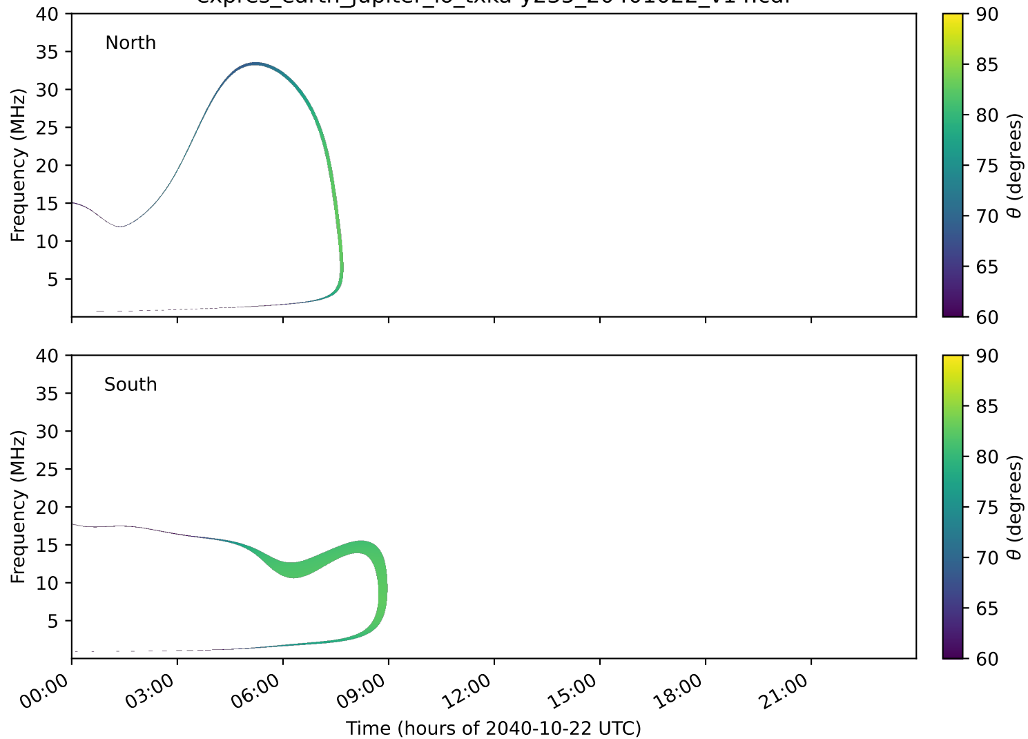
expres_earth_jupiter_io_txka-y235_20401022_v14.cdf
