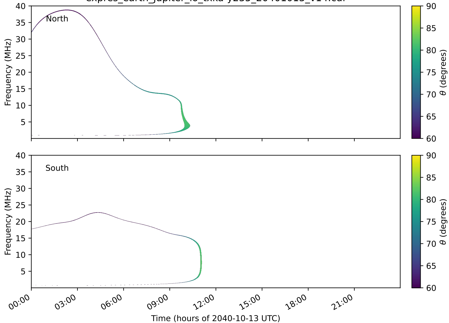
expres_earth_jupiter_io_txka-y235_20401013_v14.cdf
