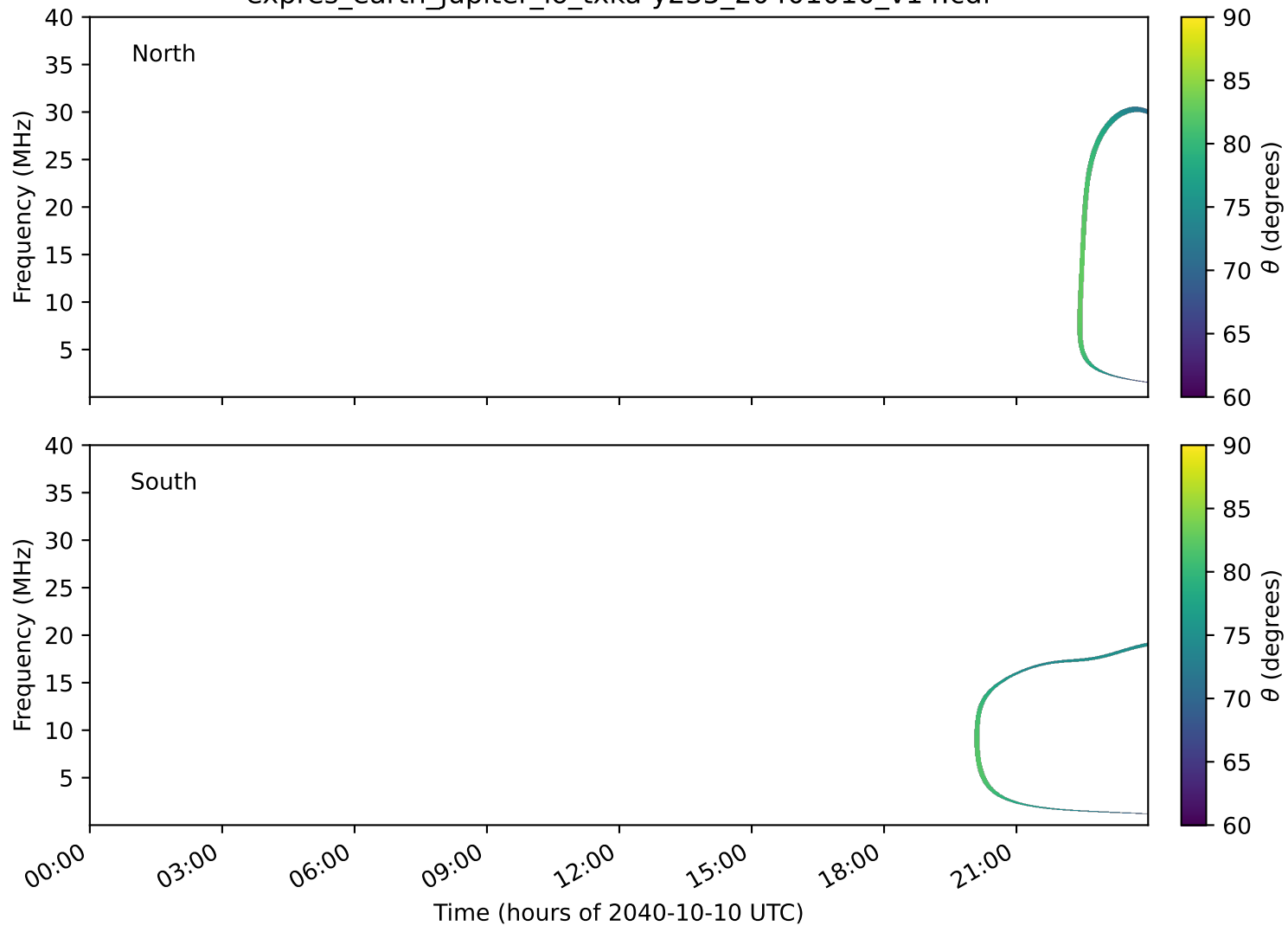
expres_earth_jupiter_io_txka-y235_20401010_v14.cdf
