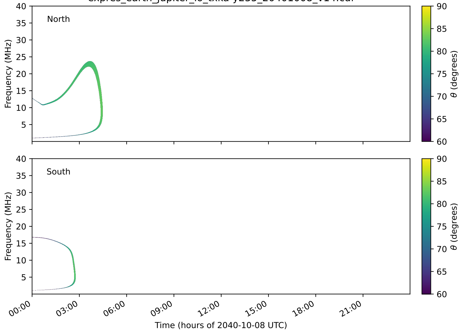
expres_earth_jupiter_io_txka-y235_20401008_v14.cdf
