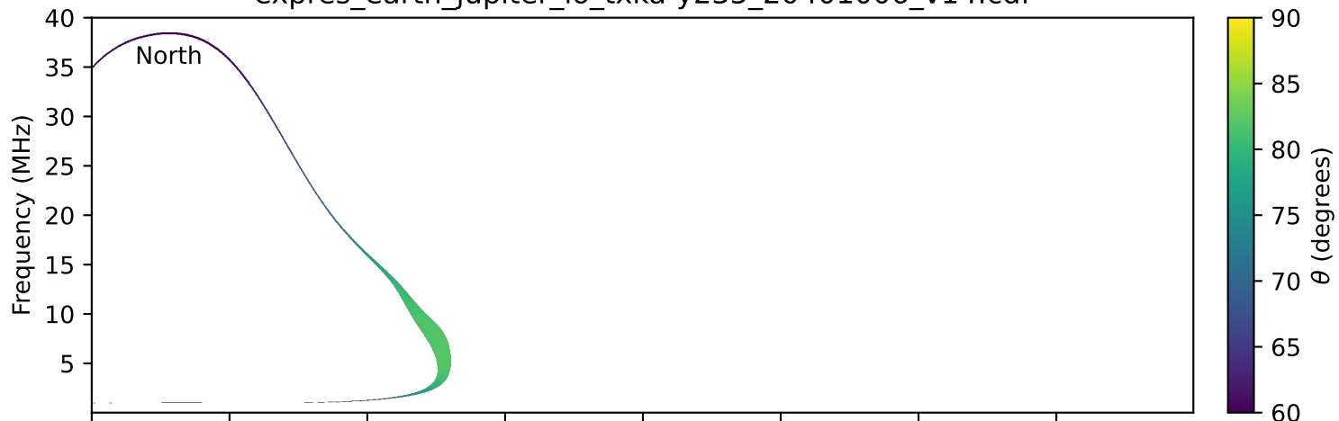
expres_earth_jupiter_io_txka-y235_20401006_v14.cdf
