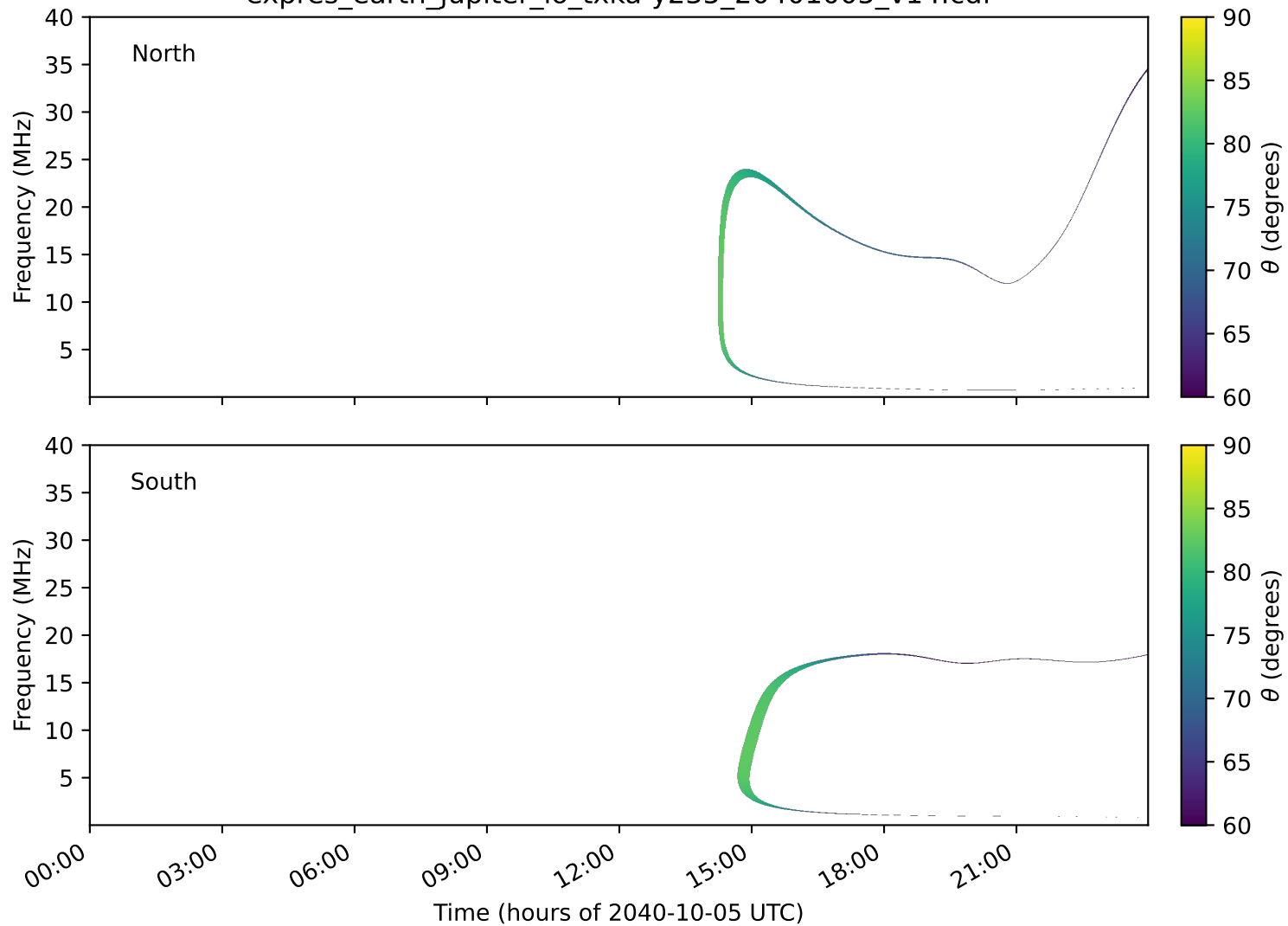
expres_earth_jupiter_io_txka-y235_20401005_v14.cdf
