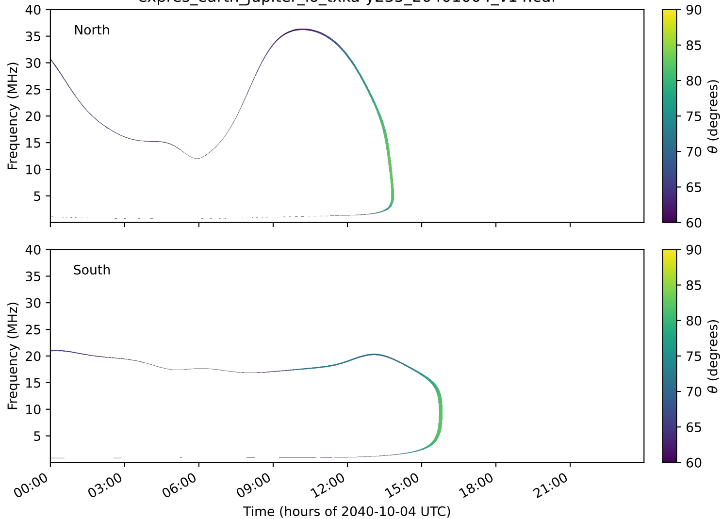
expres_earth_jupiter_io_txka-y235_20401004_v14.cdf
