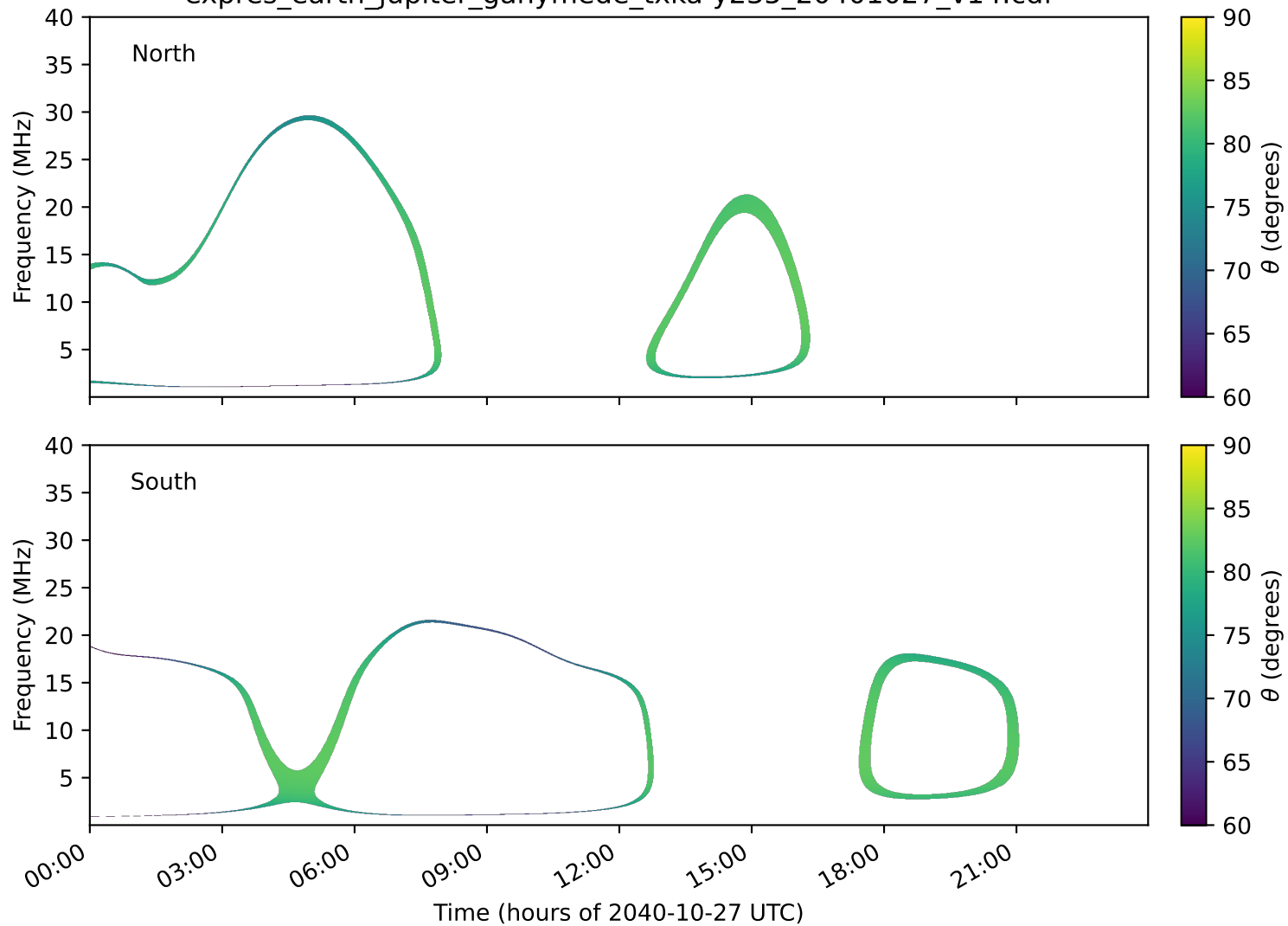
expres_earth_jupiter_ganymede_txka-y235_20401027_v14.cdf
