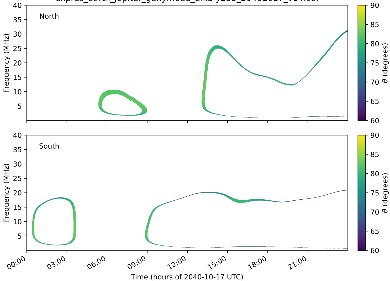
expres_earth_jupiter_ganymede_txka-y235_20401017_v14.cdf
