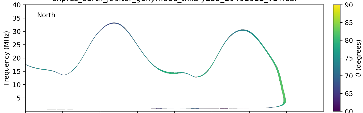
expres_earth_jupiter_ganymede_txka-y235_20401012_v14.cdf
