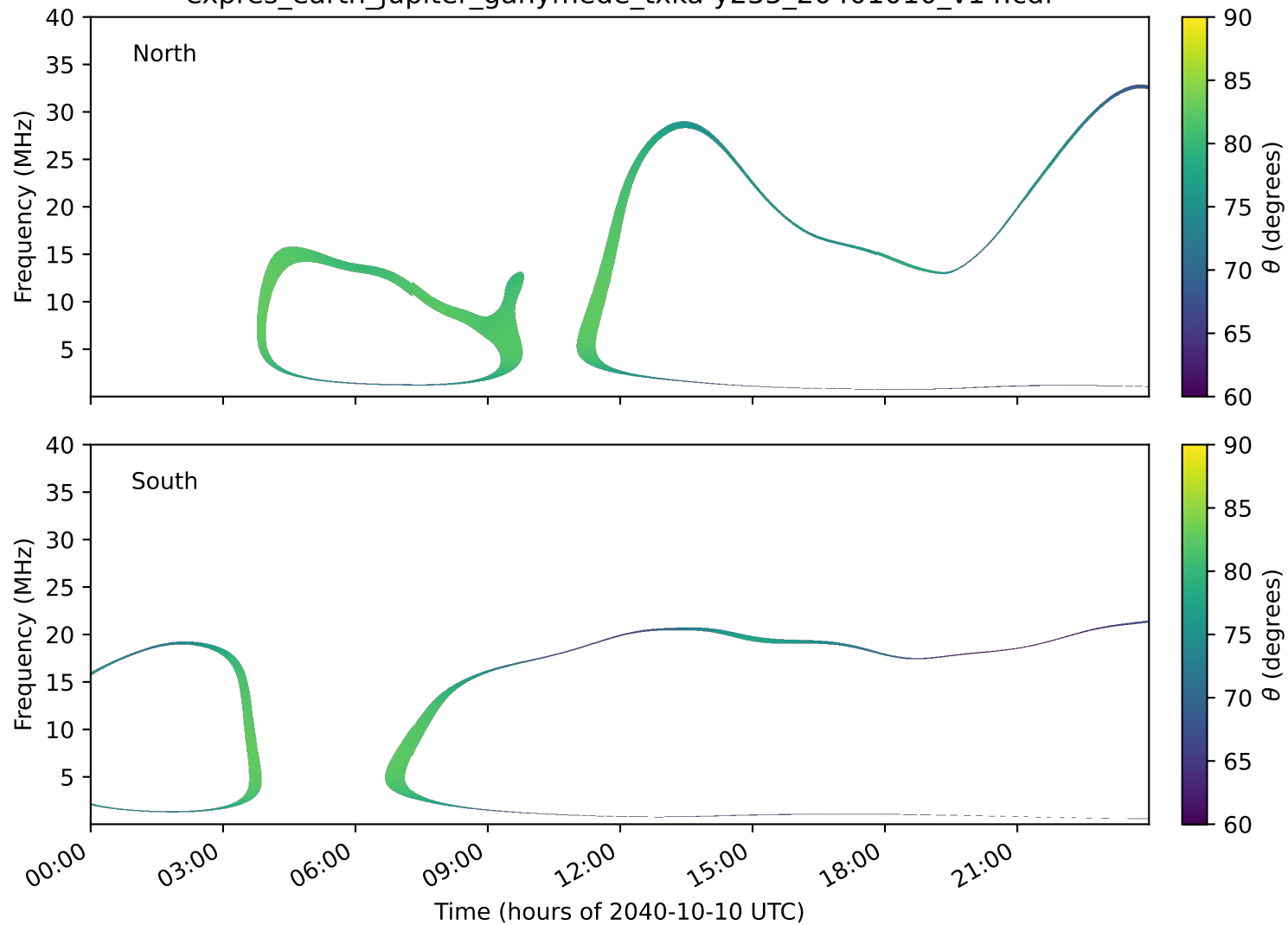
expres_earth_jupiter_ganymede_txka-y235_20401010_v14.cdf
