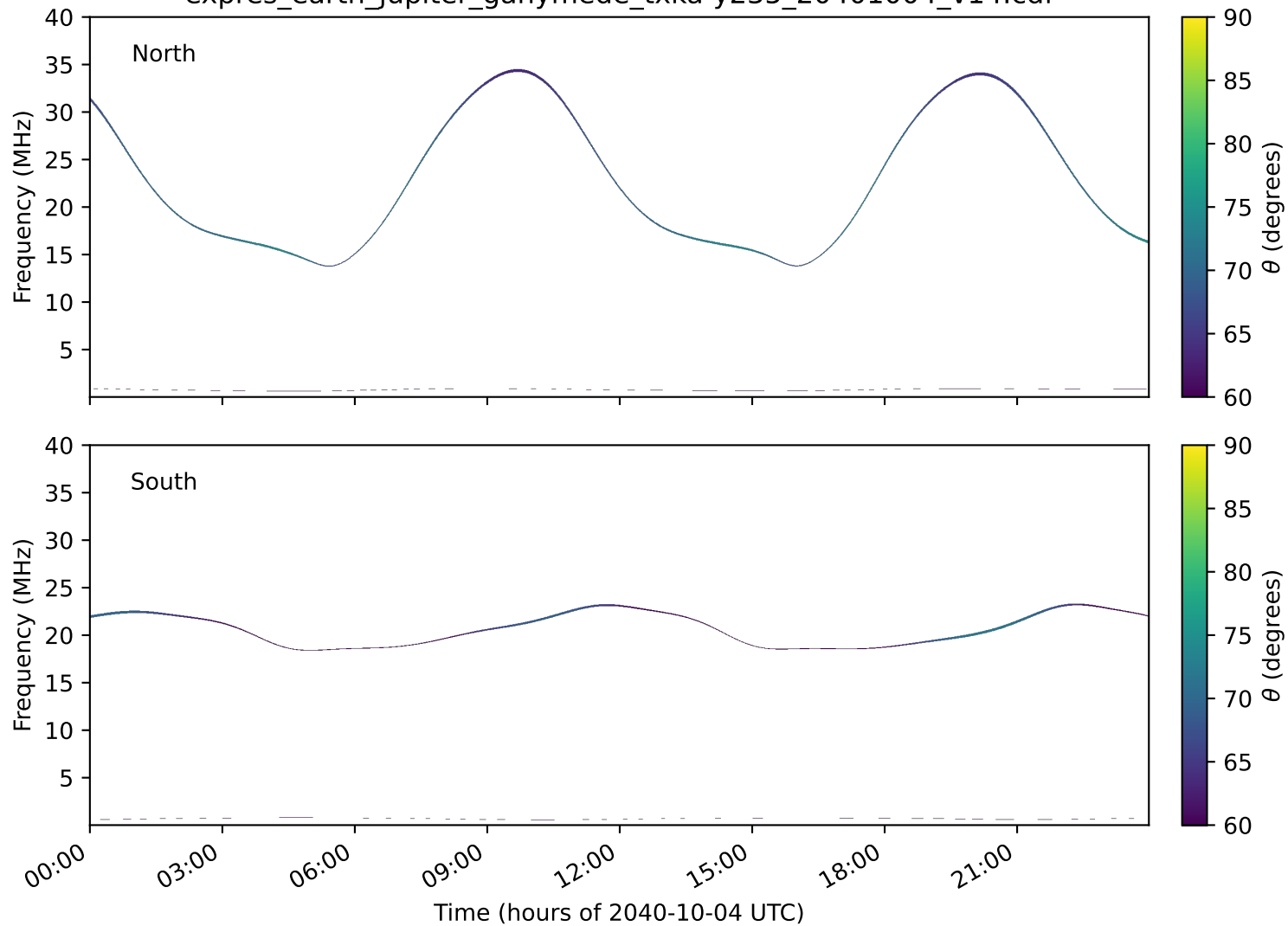
expres_earth_jupiter_ganymede_txka-y235_20401004_v14.cdf
