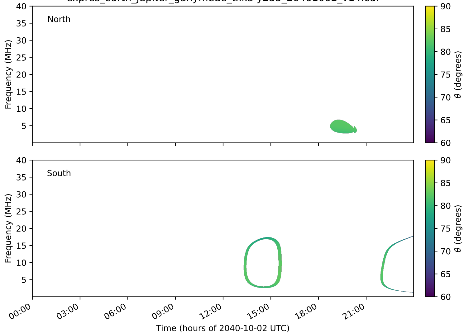
expres_earth_jupiter_ganymede_txka-y235_20401002_v14.cdf
