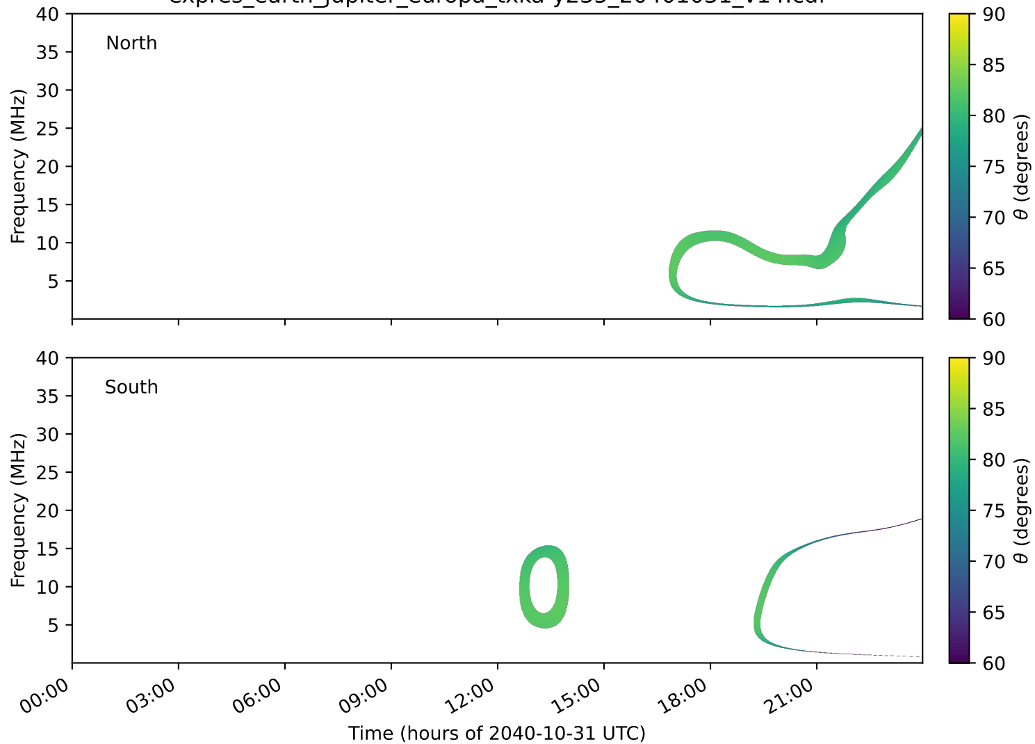
expres_earth_jupiter_europa_txka-y235_20401031_v14.cdf
