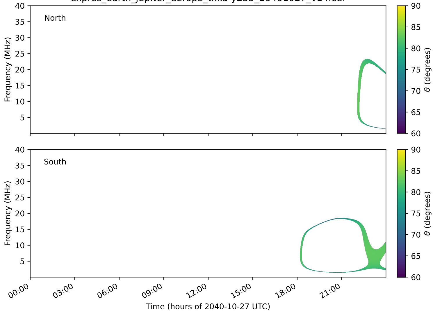
expres_earth_jupiter_europa_txka-y235_20401027_v14.cdf
