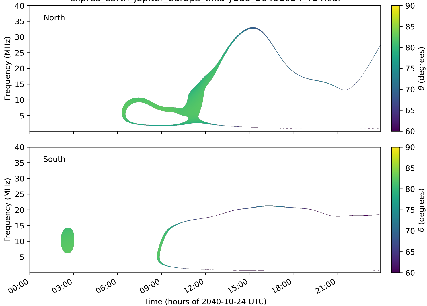
expres_earth_jupiter_europa_txka-y235_20401024_v14.cdf
