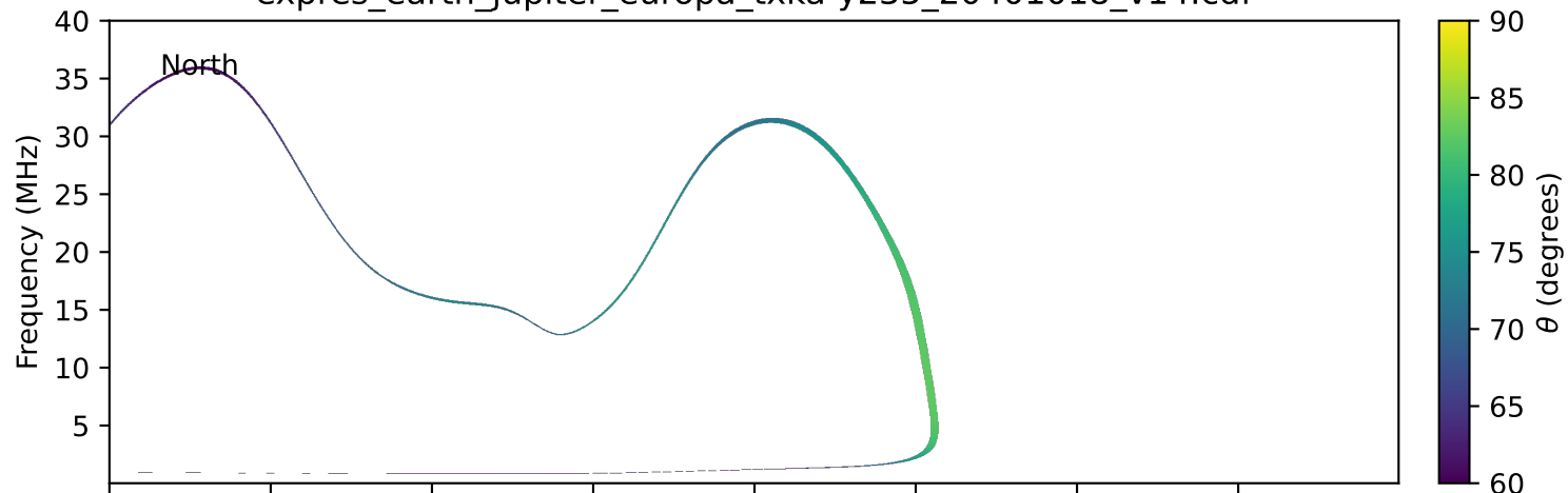
expres_earth_jupiter_europa_txka-y235_20401018_v14.cdf
