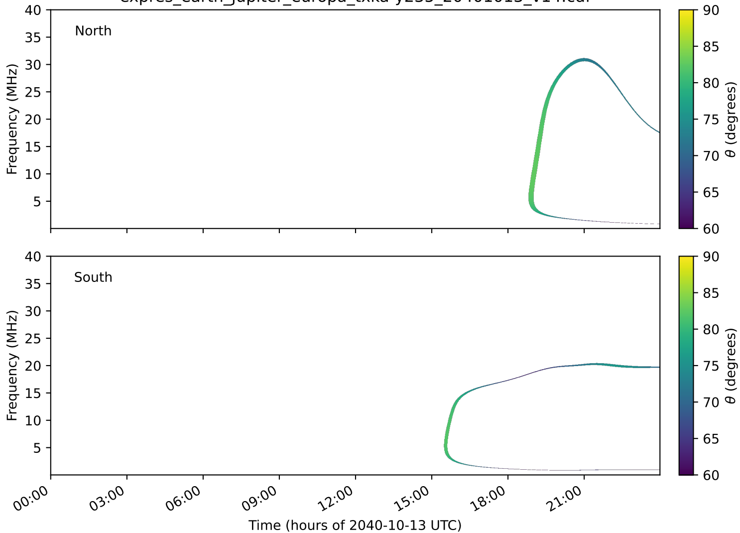
expres_earth_jupiter_europa_txka-y235_20401013_v14.cdf
