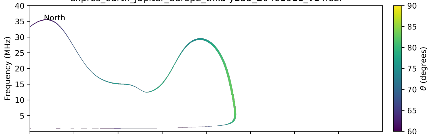
expres_earth_jupiter_europa_txka-y235_20401011_v14.cdf
