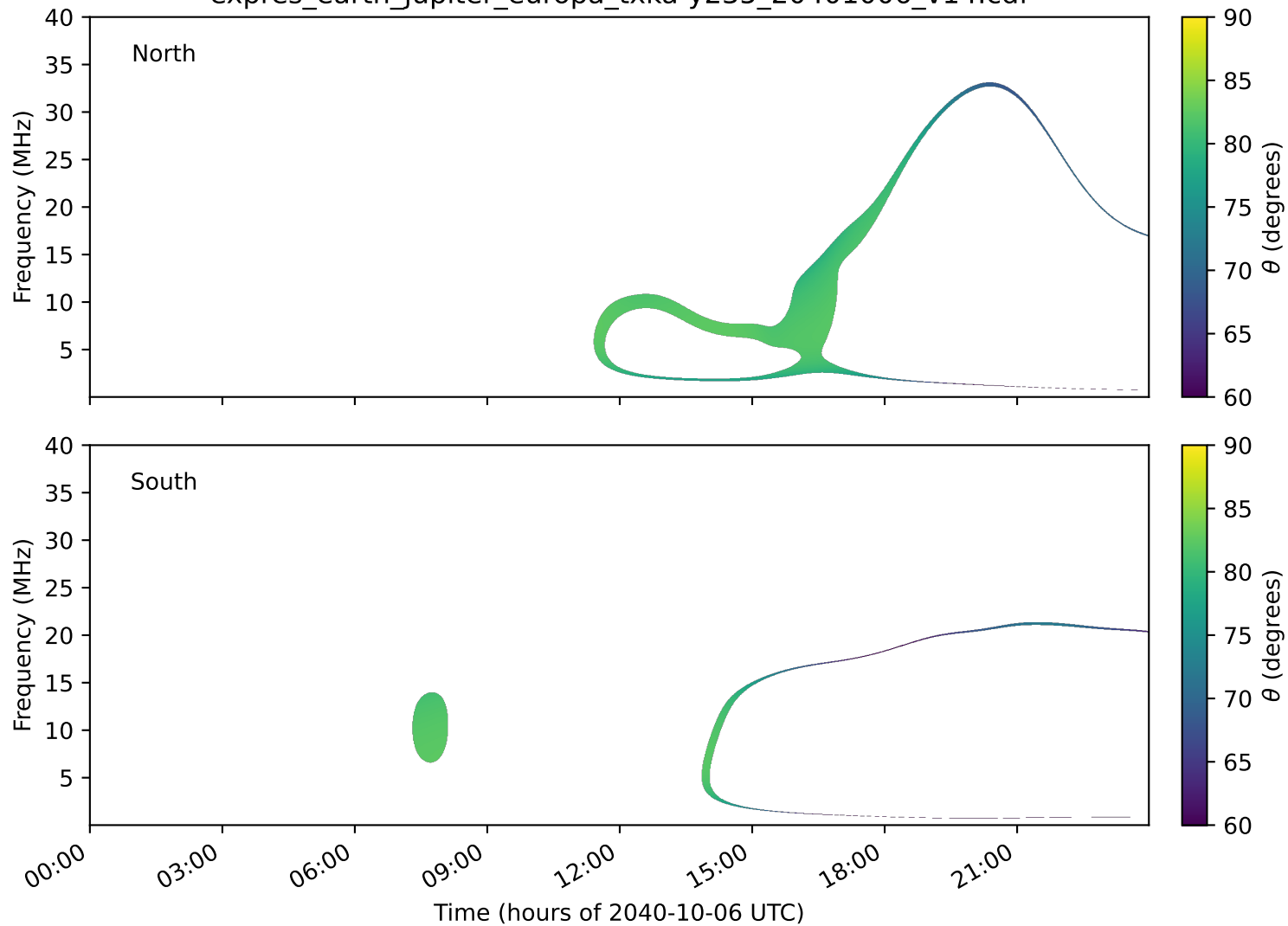
expres_earth_jupiter_europa_txka-y235_20401006_v14.cdf
