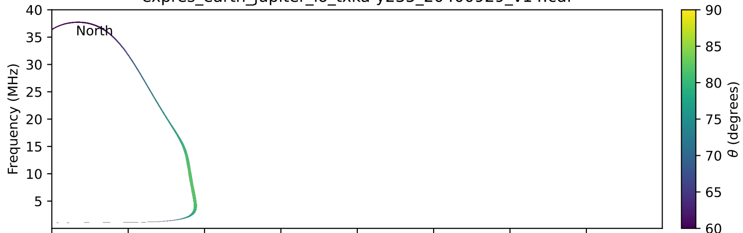
expres_earth_jupiter_io_txka-y235_20400929_v14.cdf
