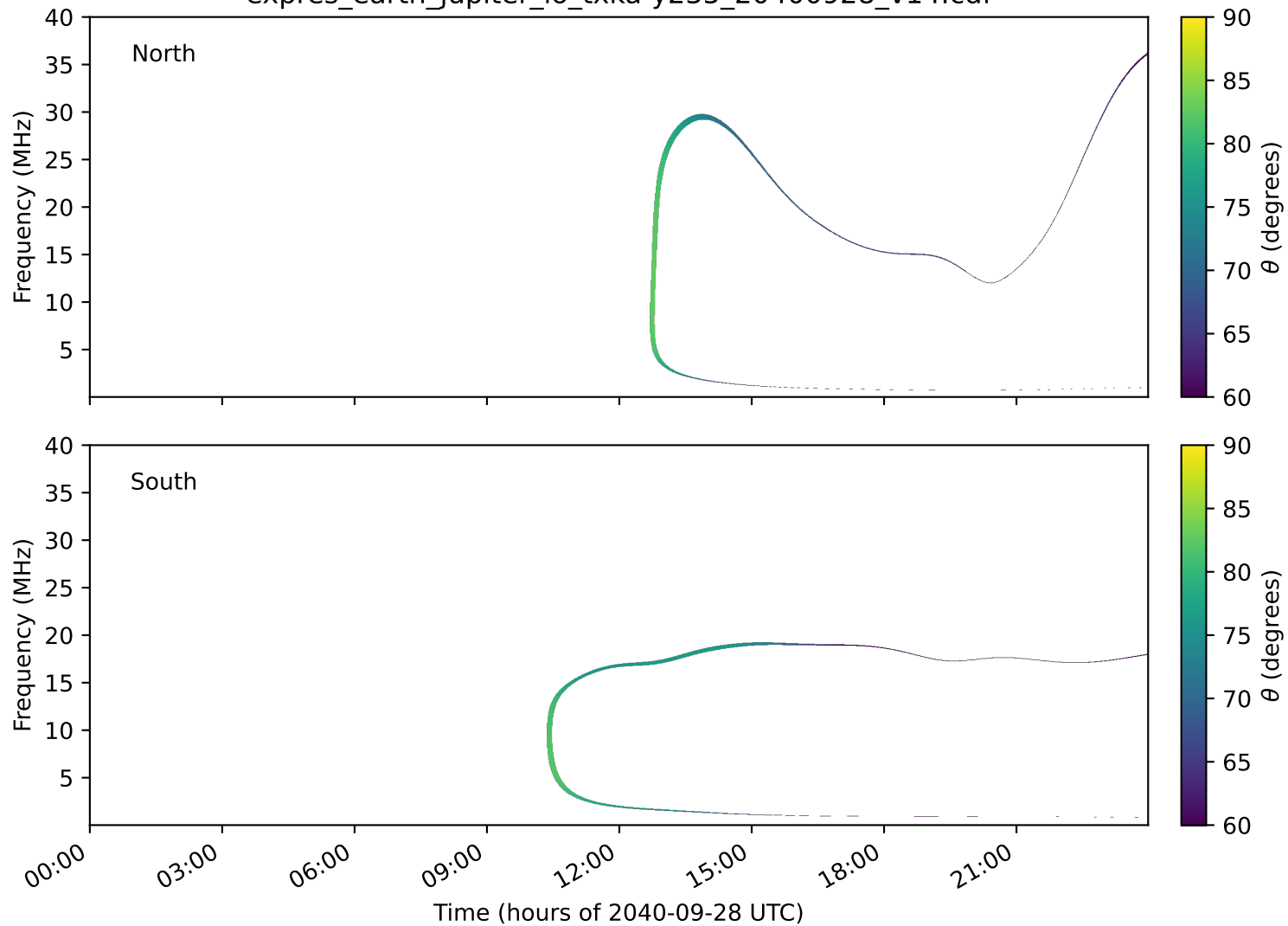
expres_earth_jupiter_io_txka-y235_20400928_v14.cdf
