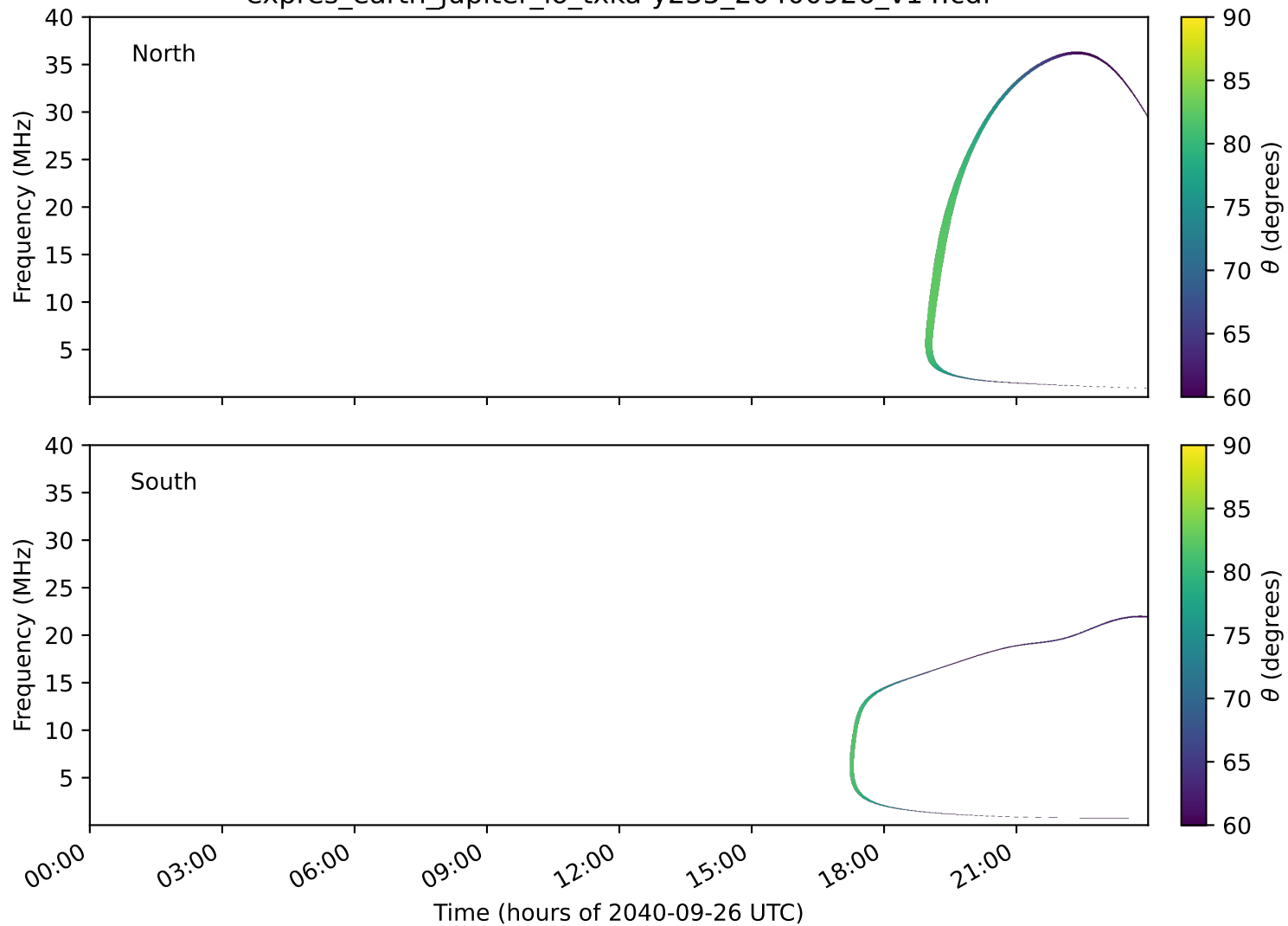
expres_earth_jupiter_io_txka-y235_20400926_v14.cdf
