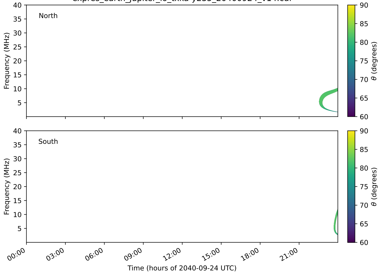
expres_earth_jupiter_io_txka-y235_20400924_v14.cdf
