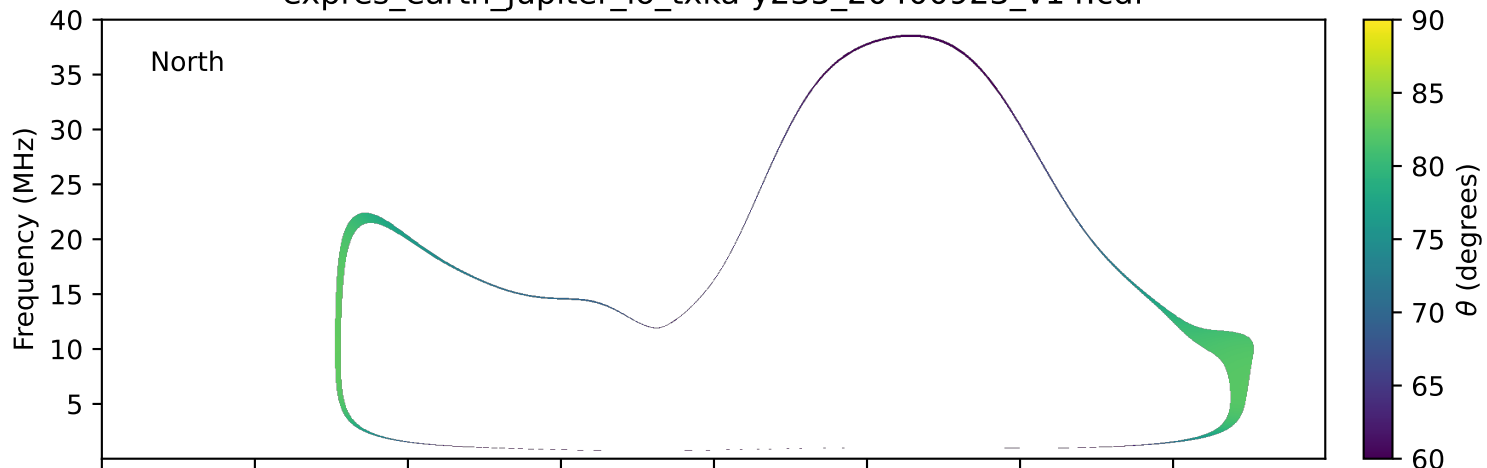
expres_earth_jupiter_io_txka-y235_20400923_v14.cdf
