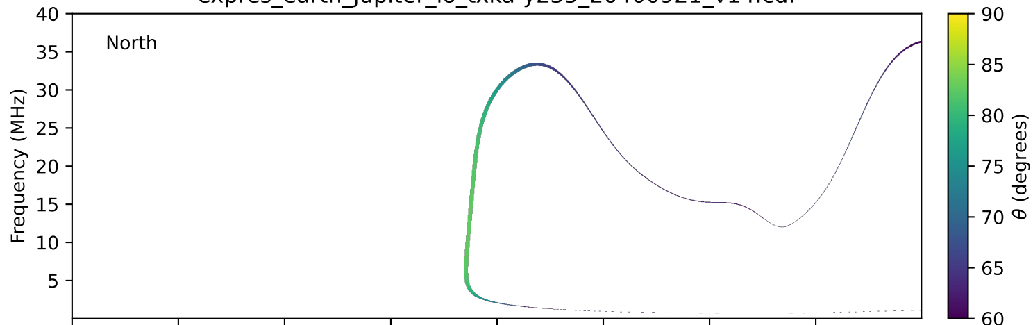
expres_earth_jupiter_io_txka-y235_20400921_v14.cdf
