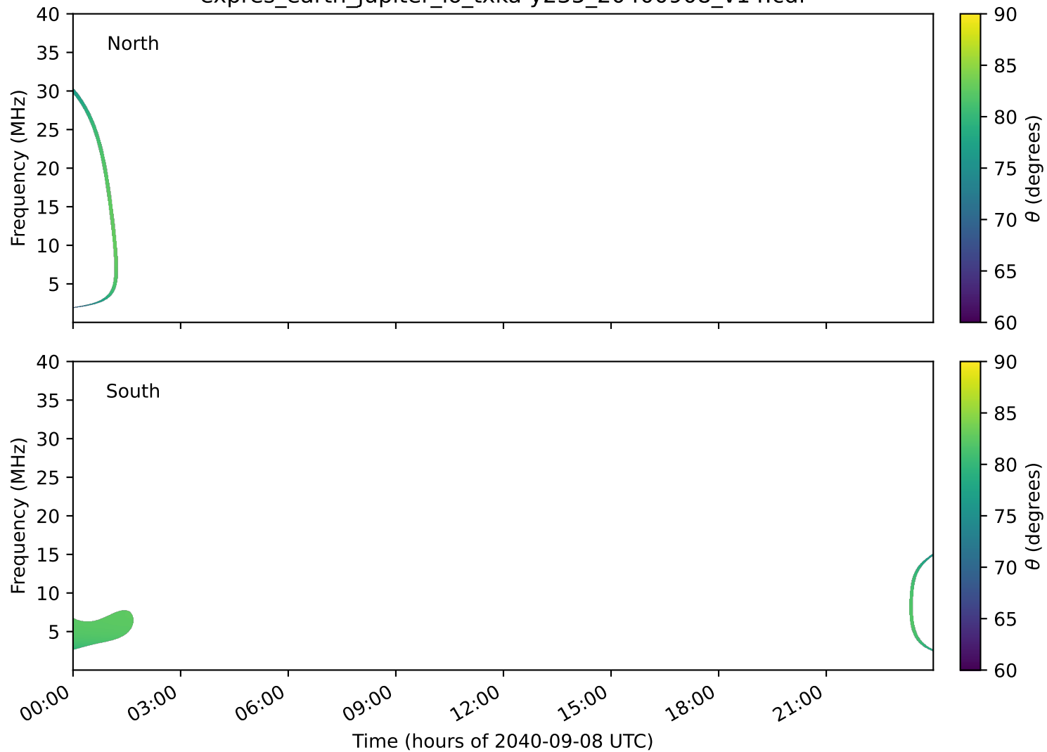
expres_earth_jupiter_io_txka-y235_20400908_v14.cdf
