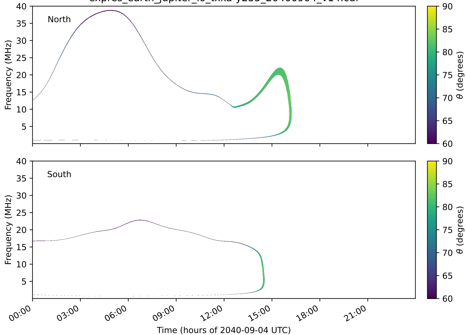
expres_earth_jupiter_io_txka-y235_20400904_v14.cdf
