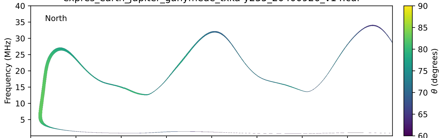
expres_earth_jupiter_ganymede_txka-y235_20400926_v14.cdf
